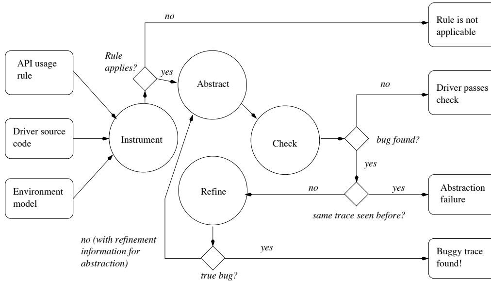
Figure 5: SDV's analysis engine's architecture
