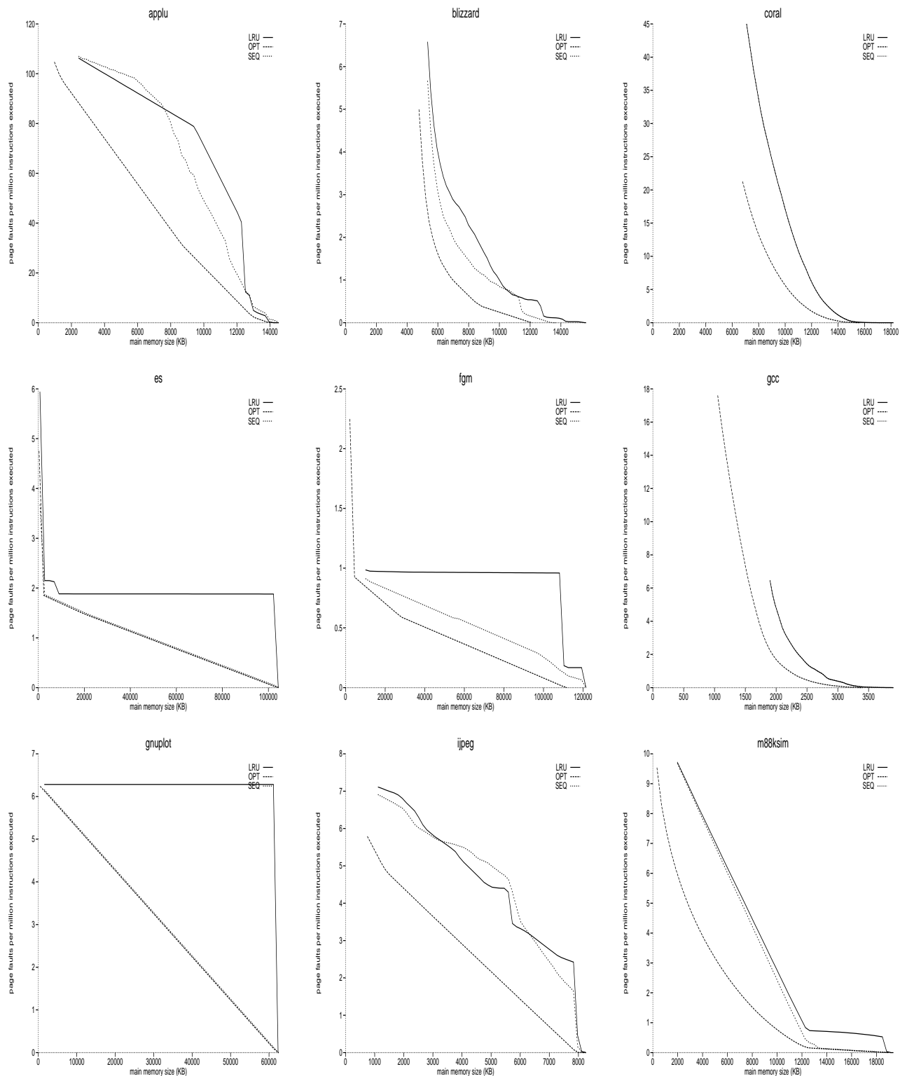
Figure 1: Performance of OPT, SEQ and LRU. For es and gnuplot , the SEQ curve almost overlaps the OPT curve. For coral and gcc , the SEQ curve overlaps the LRU curve.
