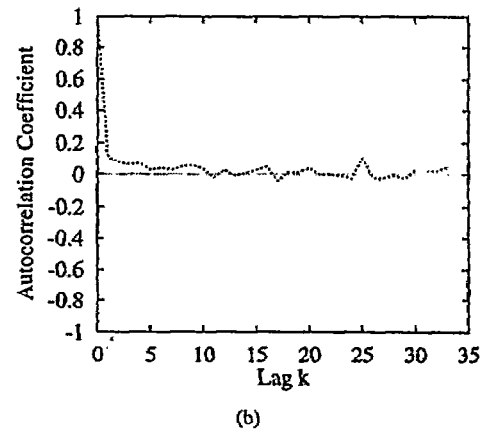
Fig. 7. Inter-reference time analysis (NASA server) (a) comparison to exponential distribution and (b) auto-correlation function.
