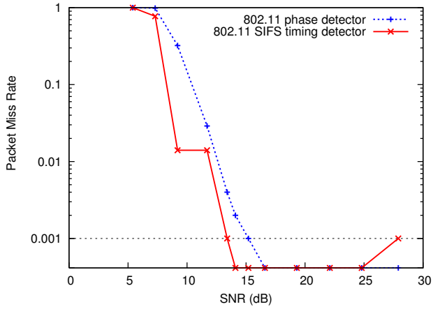
Figure 6: 802.11 unicast microbenchmark
