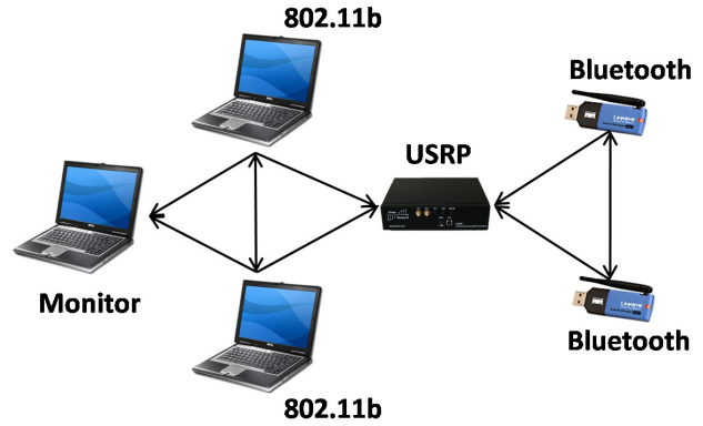
Figure 5: Configuration of nodes on the emulator
