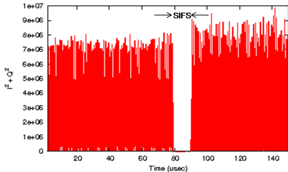
Figure 3: SIFS timing in 802.11
