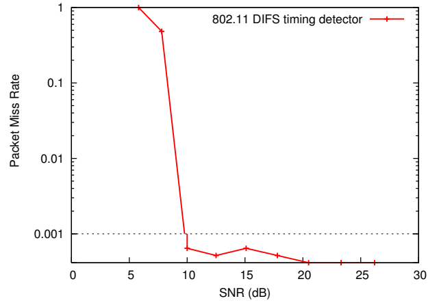
Figure 7: 802.11 broadcast microbenchmark
