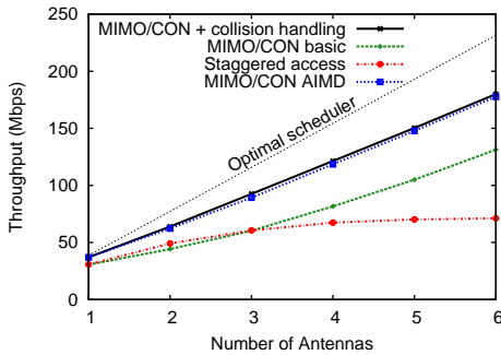
(b) PHY data rate 52Mbps
