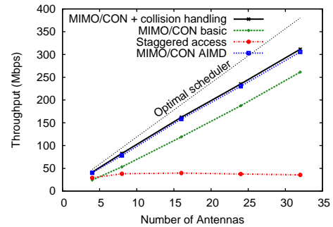
Fig. 11: Throughput of MIMO/CON with 100 nodes and PHY data rate 13Mbps.
