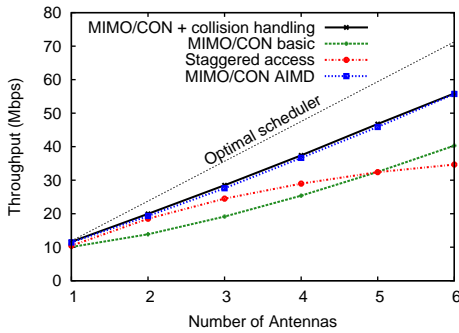
(a) PHY data rate 13Mbps
