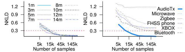
Figure 20: NKLD values wrt. to audio transmitter’s pulse distribution for (a) audio transmitter at different distances (b) different RF devices
