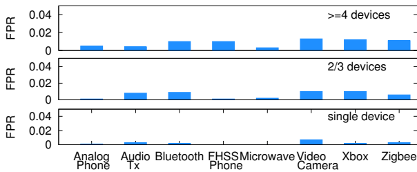
Figure 17: False positive rate for different devices.
