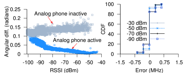
Figure 18: (a) RSSI vs. angular difference with respect to analog phone’s spectral signature when the device is switched on and off (b) CDF of bandwidth estimation error at different signal strengths.
