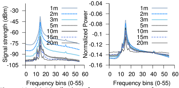
Figure 10: (a) Distribution of average power vs. frequency for an analog cordless phone at different distances. (b) Spectral signatures for the analog cordless phone are not affected for RSSI values of \geq -80 dBm.
