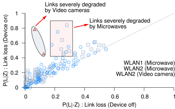
Figure 21: Results from a two day deployment of Airshark in two production WLANs. Each point in the scatter plot denotes the loss rate for a link in the absence ( p(L|\neg Z) ) and the loss rate in the presence ( p(L|Z) ) of (i) microwave ovens, (ii) video cameras, for a total of 224 links (168 links in WLAN1 and 56 links in WLAN2).
