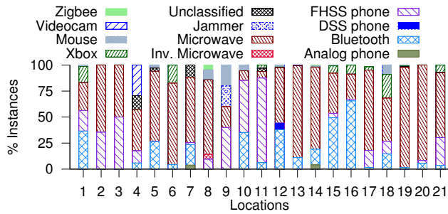
Figure 4: Distribution of non-WiFi device instances at various locations.
