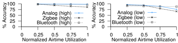
Figure 19: Stress testing Airshark with extreme WiFi interference. Detection accuracy is reduced for pulsed transmission devices (e.g., ZigBee), whereas accuracy for frequency hoppers is minimally affected.
