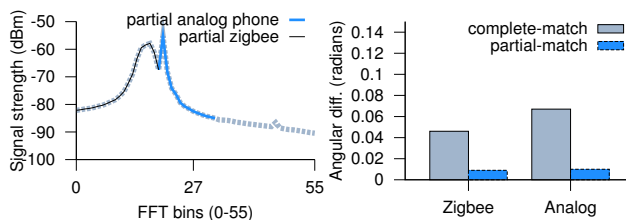
Figure 14: Overlapping signal detection. (a) partial overlap between ZigBee and analog signals (b) using partial matches between spectral signatures reduces the angular difference in overlapping cases.
