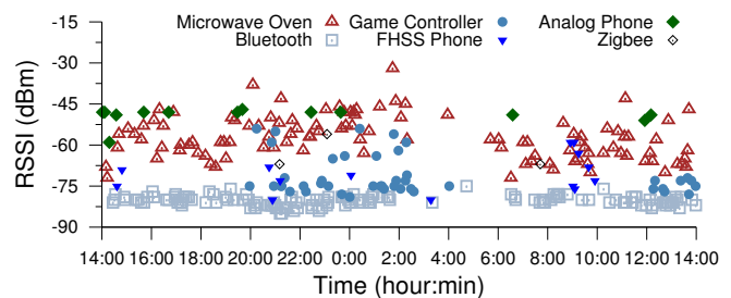
Figure 2: Average RSSI from different non-WiFi RF device instances shown against the device start times. Measurements were taken at a dorm-style apartment (location L16, dataset S2) for a 24 hour period.
