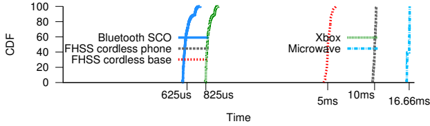
Figure 11: Inter-pulse timing signature for different devices.
