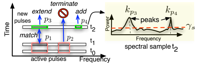
Figure 9: Illustration of the pulse detection and matching procedure. Pulse detector processes the spectral sample at time t_2 to output two new pulses p_3 and p_4 . New pulse p_3 matches with the active pulse p_1 , and results in extending p_1 . Active pulse p_2 is terminated as there is no matching new pulse, and new pulse p_4 is added to the active pulse list.
