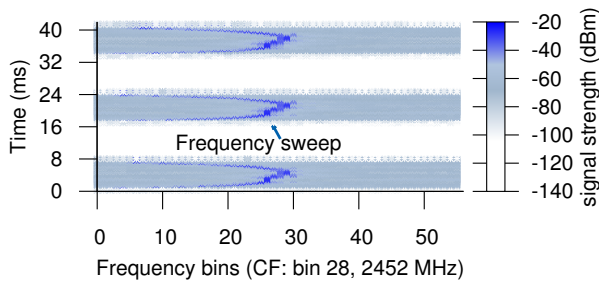
Figure 13: Spectral samples from Airshark capturing the activity of a residential microwave. The plot shows (i) the ON-OFF cycle for is around 16.6 ms and (ii) “frequency sweeps” during the ON periods.
