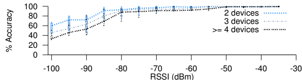
Figure 16: Accuracy of detection across signal strengths for 2, 3, and \geq 4 device combinations.
