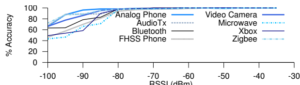
Figure 15: Accuracy of single device detection across signal strengths for different RF devices.
