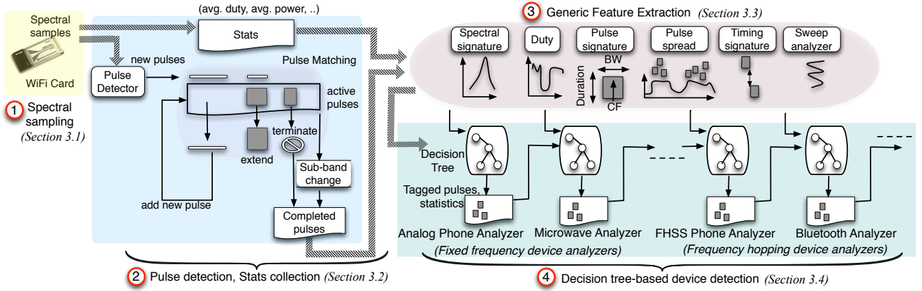
Figure 8: (a) Illustration of Airshark’s detection pipeline. Spectral samples from the WiFi card are generated using a scanning procedure (§3.1). These samples are processed to detect signal pulses , and collect some aggregate statistics based on the received power values (§3.2). In the next stage, various features capturing the spectral and temporal properties of the signals are extracted (§3.3), and are used by different device analyzers that employ decision tree models (§3.4) trained to detect their target RF devices.
