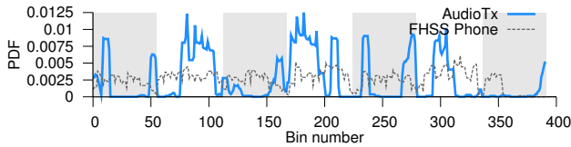
Figure 12: Pulse distribution of FHSS cordless phone and an audio transmitter as captured by Airshark.
