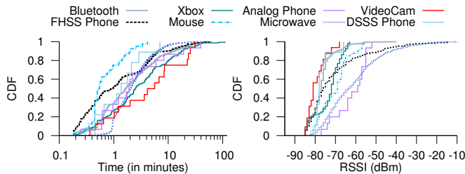
Figure 5: Distribution of (a) Session durations of the non-WiFi device instances (X-axis in log-scale) and (b) RSSIs of the non-WiFi device instances aggregated across all locations.
