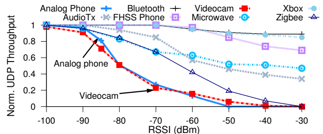
Figure 1: Degradation in UDP throughput of a good quality WiFi link (WiFi transmitter and receiver were placed 1m apart) in the presence of non-WiFi devices operating at different signal strengths.
