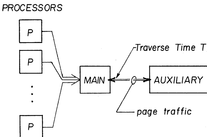
FIG. 1. Two-level memory system
