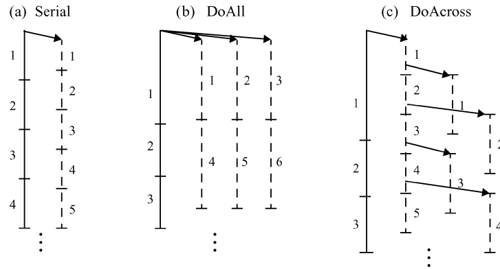
Fig. 5. Three pre-execution thread initiation schemes: (a) SERIAL, (b) DoAll, and (c) DoAcross. Solid lines denote the main thread, dotted lines denote pre-execution threads, arrows denote thread spawning, and numeric labels denote loop iteration counts.
