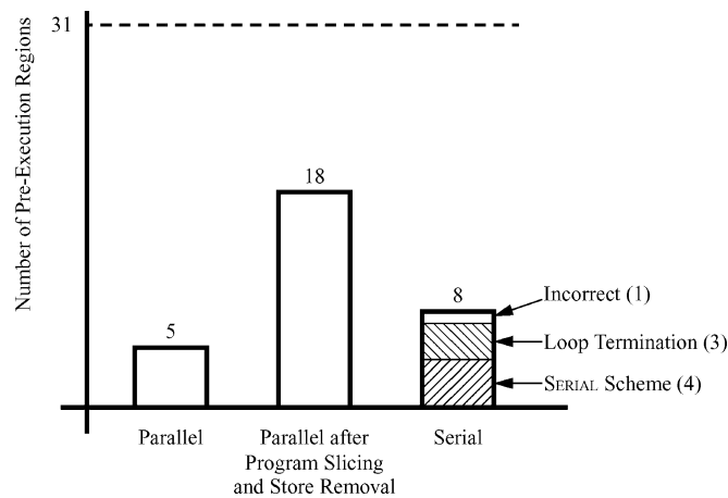
Fig. 12. Breakdown of pre-execution regions into three major categories: originally parallel, parallel after program slicing and store removal, and serial. The serial category is further broken down into regions using the SERIAL scheme, regions speculatively parallelized affecting control flow only, and regions that are incorrectly parallelized.
