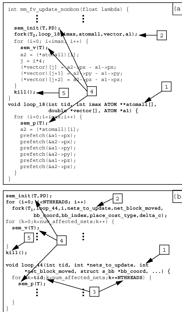
Fig. 7. Code generated by the aggressive compiler to implement the (a) SERIAL scheme for the AMMP benchmark, and (b) DOALL scheme for the VPR benchmark. Code for initiating pre-execution and synchronizing pre-execution threads appears in bold-face.
