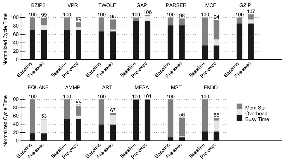
Fig. 10. Normalized execution time broken down into busy, overhead, and memory stall components. The “Baseline” and “Pre-exec” bars show performance for no pre-execution and with pre-execution, respectively.
