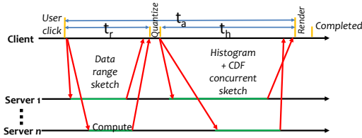
Figure 7: Execution timeline for computing a histogram; diagonal arrows show messages between client and servers.
