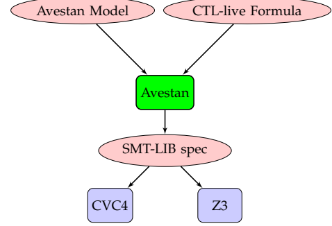
Fig. 7. Overview of our method
