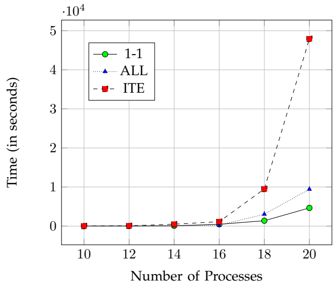
Fig. 12. Z3 on different models for the leader election problem
