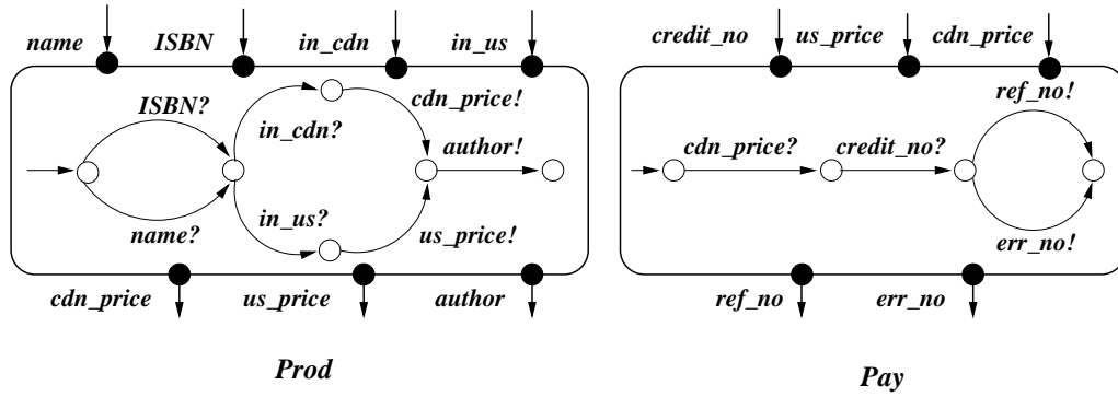
Fig. 1: Two IAs: Prod and Pay .
