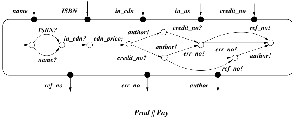
Fig. 4: Prod // Pay is the composition of two composable IAs in Figure 1.
