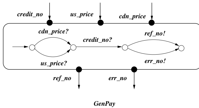
Fig. 5: GenPay refines Pay in Figure 1.
