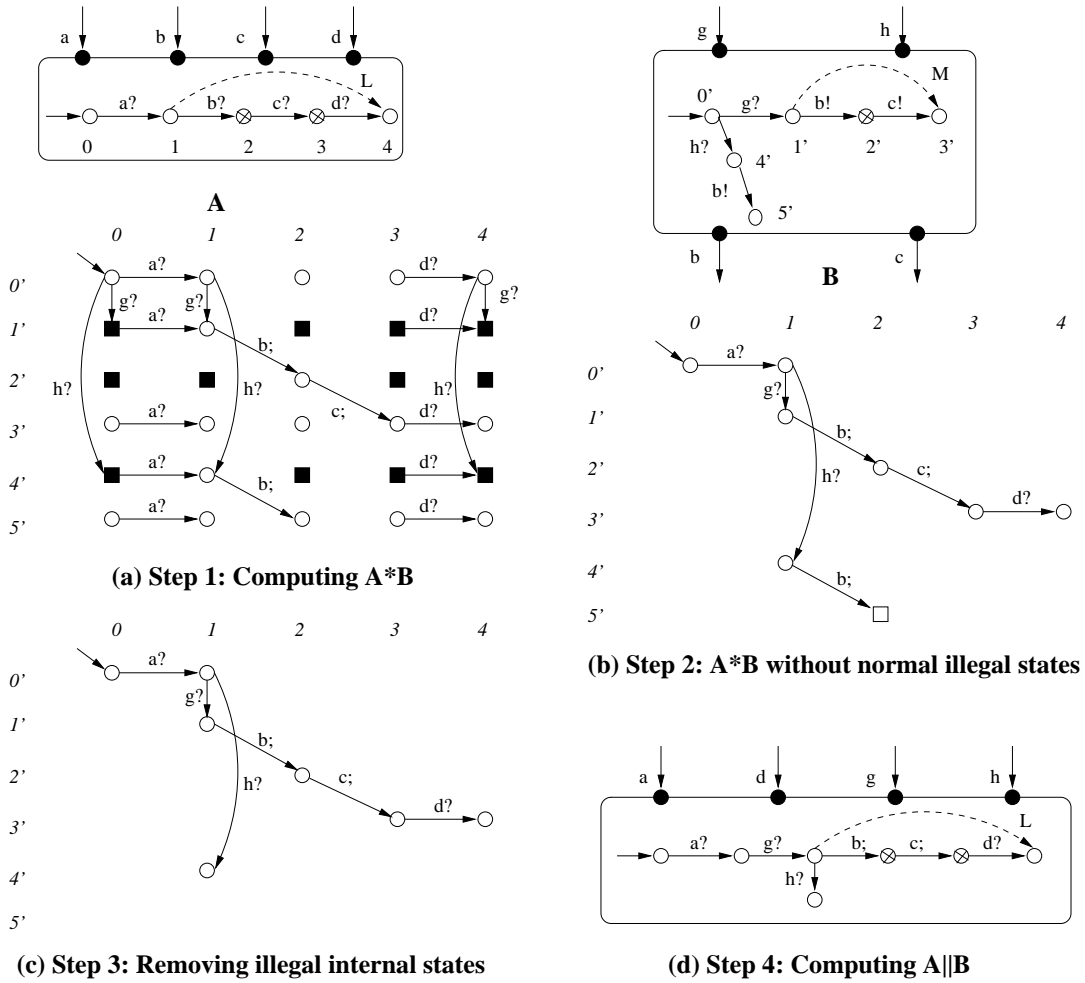
Fig. 8: Computing IACA composition for two composable IACAs.
