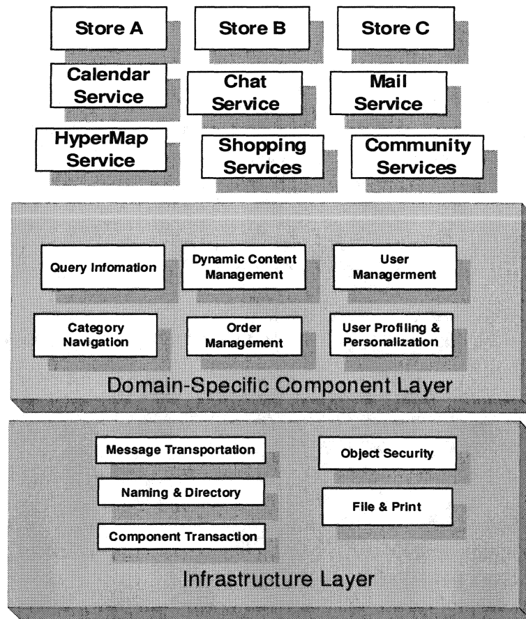
Figure 1 CIS Application Framework
