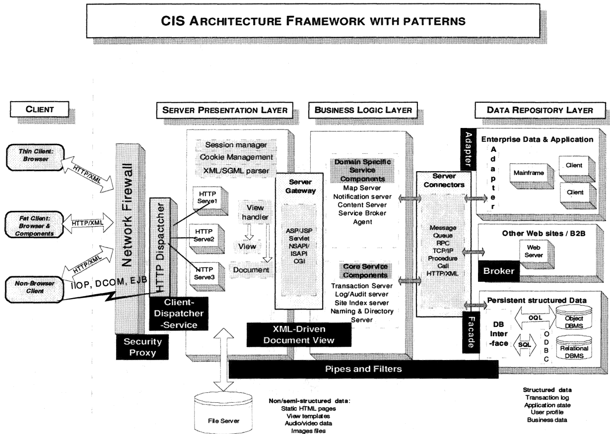
Figure 3 CIS Architecture Framework with Patterns
