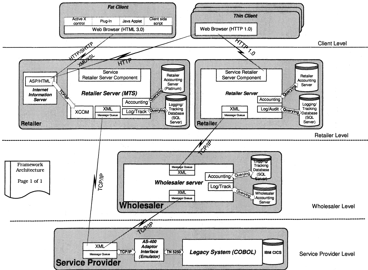
Figure 13 CB System Architecture Model
