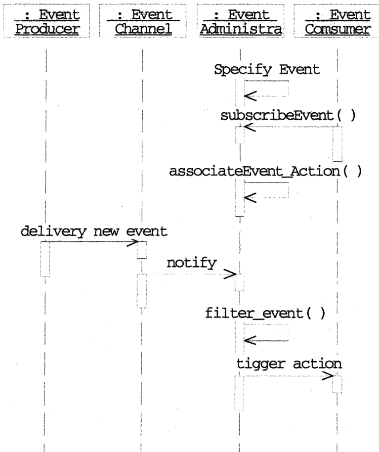
Figure 9 Sequence Diagram: Pure Push Event Model
