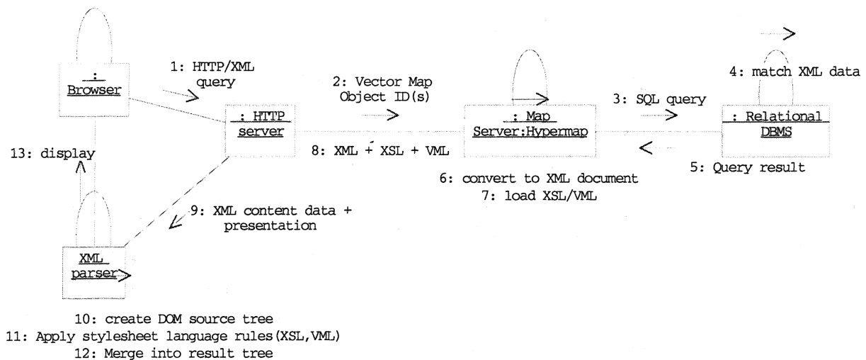
Figure 11 Collaboration Diagram: Retrieve Map Information
