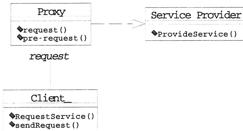
Figure 7 Class Diagram: Proxy Pattern
