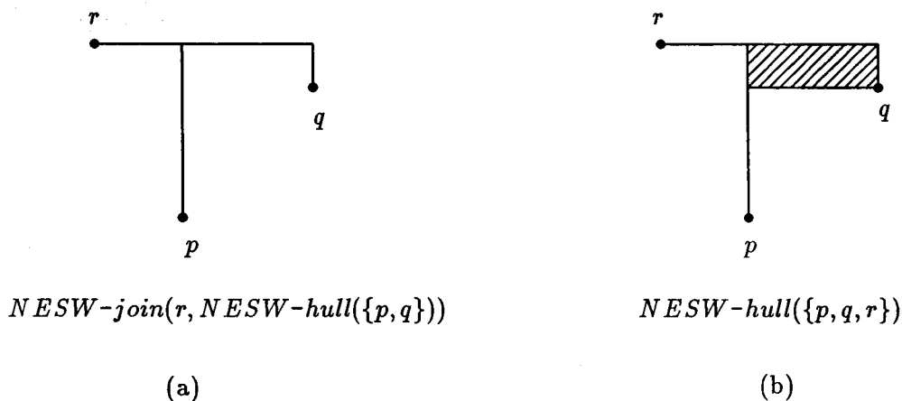
Figure 5: The NESW-join of three points.
