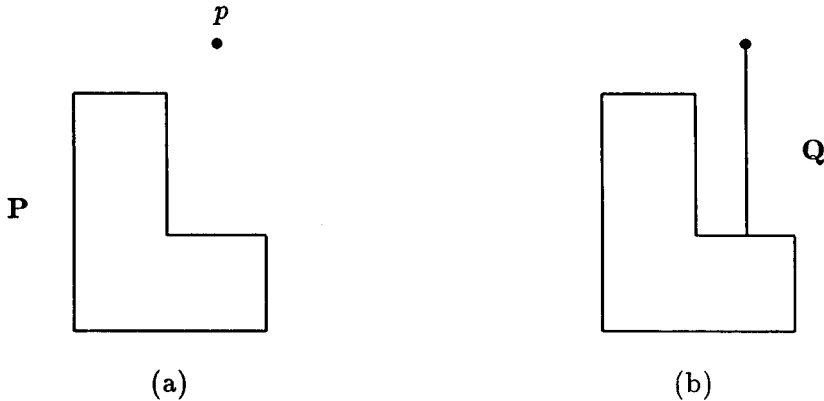
Figure 1: The join of an ortho-convex set and a point.
