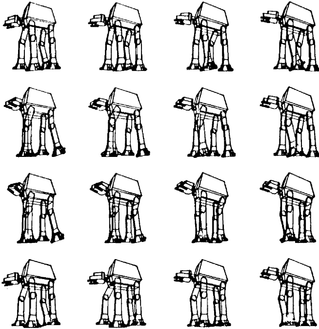
Figure 10 Zoom-pan-scroll Data
