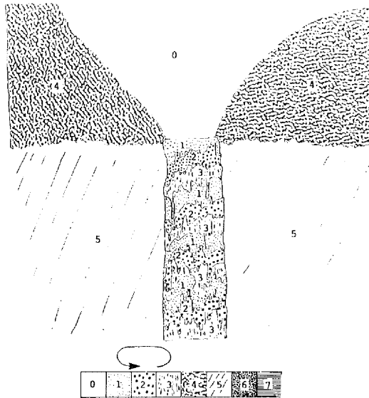
Figure 6 Colour Cycling
