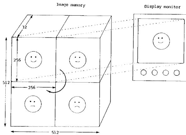
Figure 9 Zoom-pan-scroll Animation
