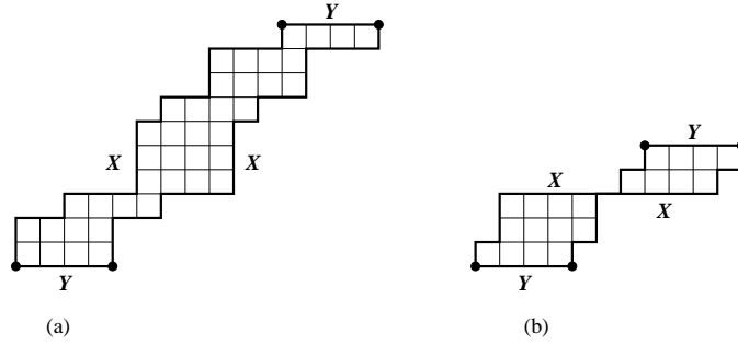
Figure 4: Examples of a polyomino in \mathcal{PSP}_{24,4}^- (a), and a polygon which is not a polyomino, (b)
