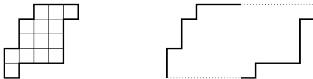
Figure 1: A parallelogram polyomino, its upper and lower paths.
