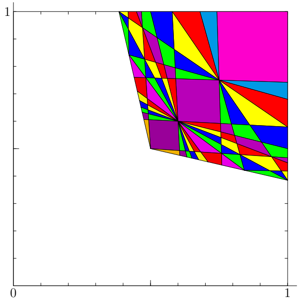
Fig. 32: Kernel=24; \mathfrak{d} = 12 , \mathfrak{c} = 3 .
