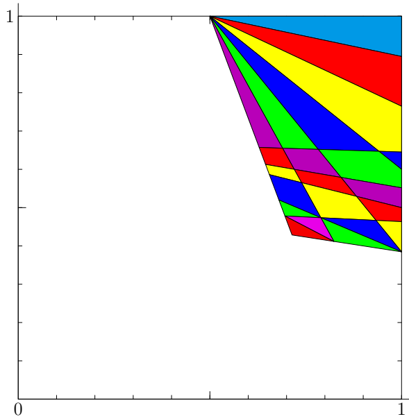
Fig. 31: Kernel=21; \mathfrak{d} = 12 , \mathfrak{c} = 3 .
