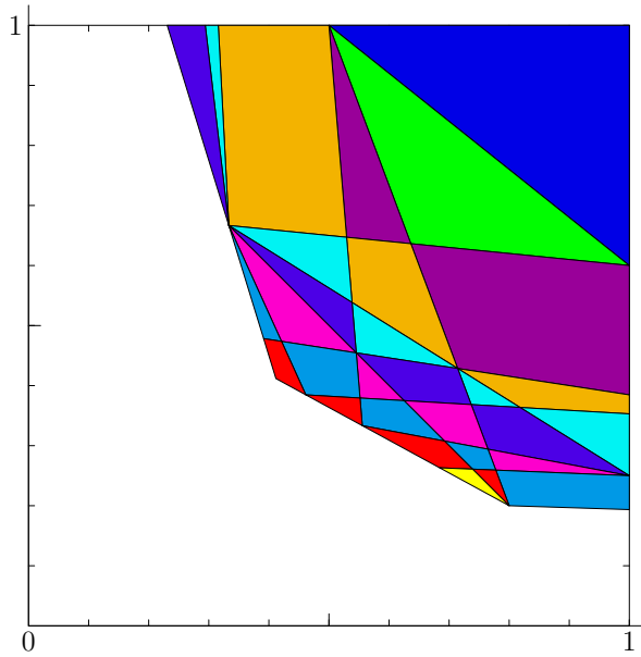
Fig. 8: Kernel=7; \mathfrak{d} = 5 , \mathfrak{c} = 1, 2, 3 or 4 . The mosaic NP_3[2, 2, 3] .
