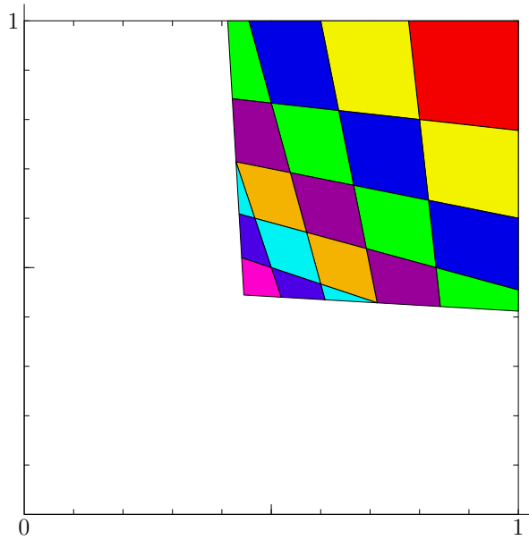
Fig. 9: Kernel=8; \mathfrak{d} = 5 , \mathfrak{c} = 1, 2, 3 or 4 . The mosaic SQ_1[8] .
