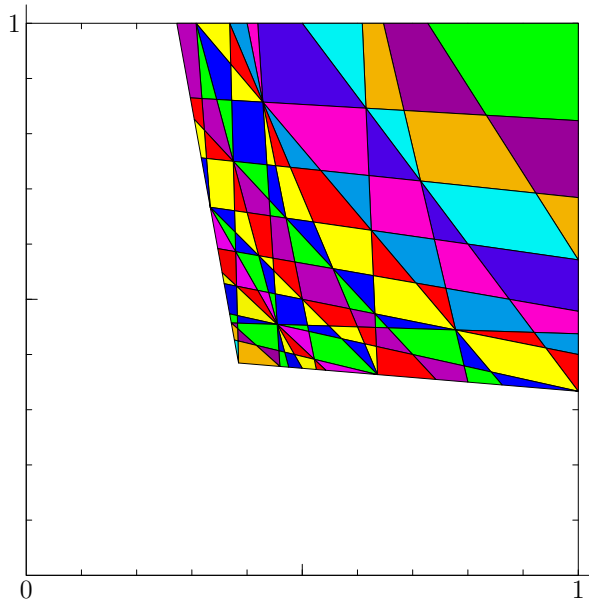
Fig. 23: Kernel=15; \mathfrak{d} = 12 , \mathfrak{c} = 3 . The mosaic NQ_4[3, 2, 1, 10] .
