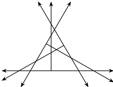
Figure 28: Three constrained long-legged \overline{T} ’s can divide the plane into 19 regions. It is impossible to add a fourth \overline{T} that meets each of the first three in 4 points.
