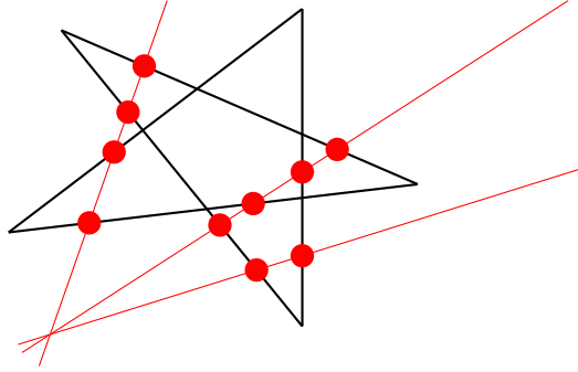
Figure 38: No line can intersect a pentagram in more than four points.
