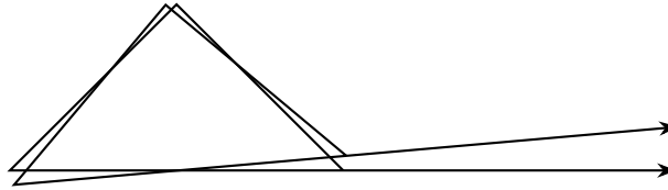
Figure 19: Two wynnns can intersect in 7 points and divide the plane into 10 regions.
