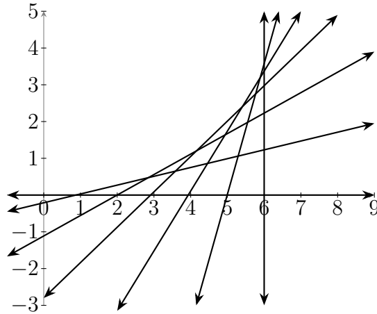
Figure 4: An optimal pancake graph G_{\mathbf{K}}(7) defined by (9) with n = 6 and \theta = 15^\circ . The t = 0 line is the x -axis, and the t = 6 line is x = 6 .
