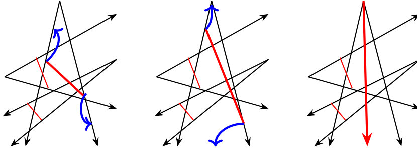
Figure 15: Converting an optimal graph with n long-legged A 's (left) into a graph with n 3-armed V 's (right). The steps do not decrease the number of regions. Reversing the last step (going from right to center) performs the inverse operation.
