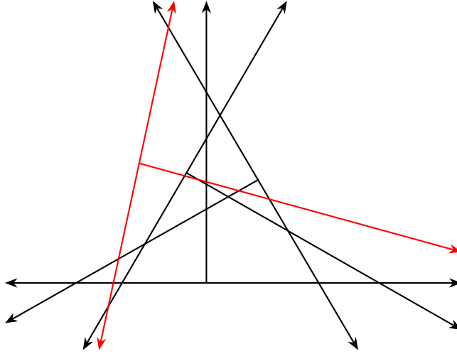
Figure 29: Four constrained long-legged \overline{T} 's can divide the plane into 32 regions. The first three are the same as in Fig. 28, and the fourth (which meets one of the first three in only three points, not four) is drawn in red.
