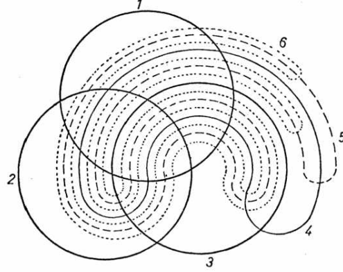
Figure 2: A 6-set Venn diagram (with 64 regions) constructed from six copies of a sausage shape S , from Grünbaum [13]. (A circle is a very simple sausage.) The construction easily generalizes to show that at least 2^n regions can be achieved using n copies of a simple Jordan curve.
