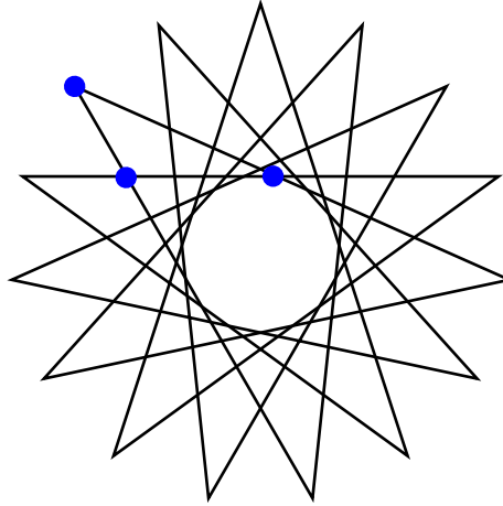
Figure 39: Three pentagrams can divide the plane into 77 regions.
