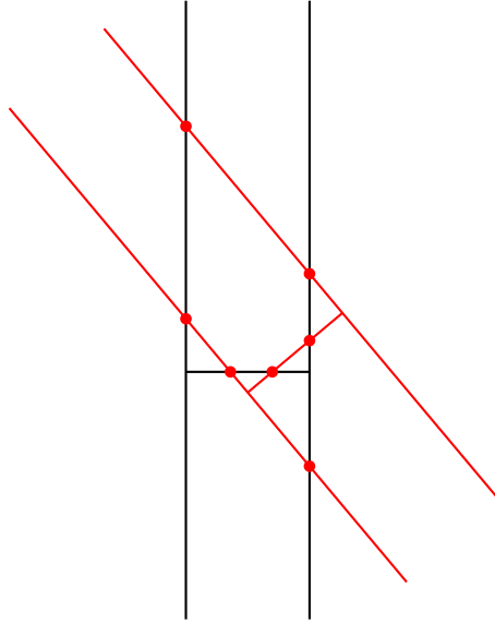
Figure 25: One of the three inequivalent ways in which two constrained \overline{H} 's can intersect in seven points.
