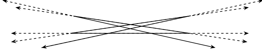
Figure 12: When an optimal chain is stellated (here, a 5-chain), only unbounded regions are added.
