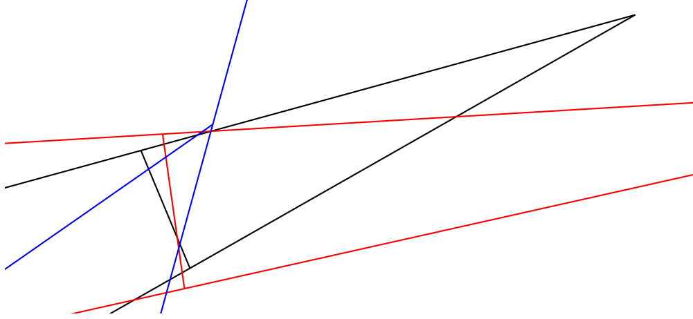
Figure 35: Enlargement of the portion of Fig. 34 where the three crossbars come together.
