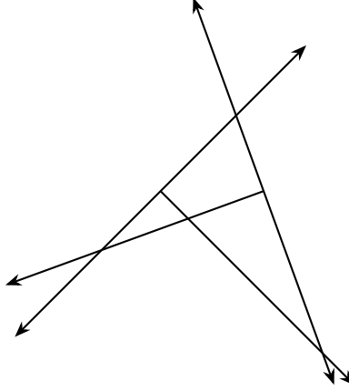
Figure 31: A good pair: two \overline{T} 's that intersect in four points. The angle between the stems must be strictly greater than \pi/2 .
