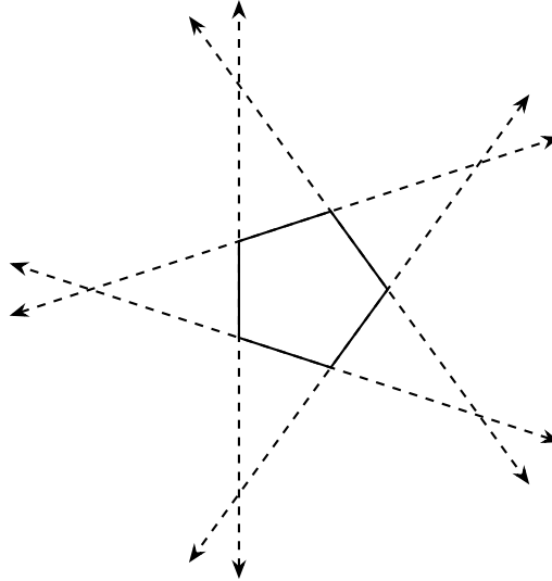
Figure 11: A pentagon and its stellation. The edges of the pentagon are replaced by lines, creating five new bounded regions and ten infinite regions.
