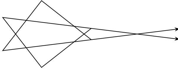
Figure 19: Two wynnns can intersect in 7 points and divide the plane into 10 regions.
