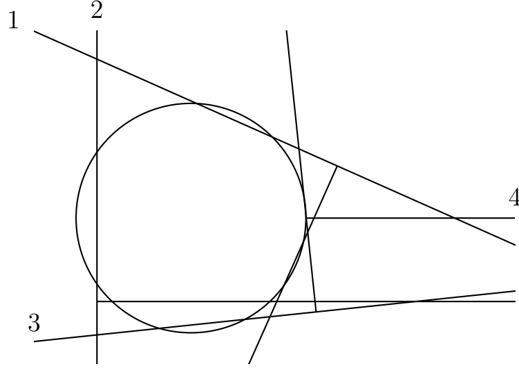
Figure 45: Enlargement of the central portion of a configuration of four lollipops with 40 intersections. Three of the lollipops are so large they appear as \overline{T} shapes. It seems unlikely, but it is true that because the lines numbered 1, 2, and 3 are actually circles, when the lines are extended, lines 1 and 2 will cross a second time, lines 1 and 3 will cross twice, and line 4 will cross line 1 a second time and will cross line 3 twice.
