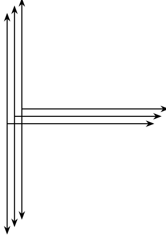
Figure 32: A step in breaking up the groups of overlaid \overline{T} 's.
