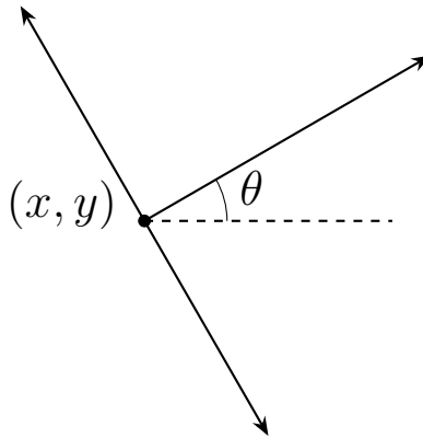
Figure 30: Parameters for a constrained long-legged \overline{T} : coordinates (x, y) of the center, and the angle \theta between the stem and the x -axis.
