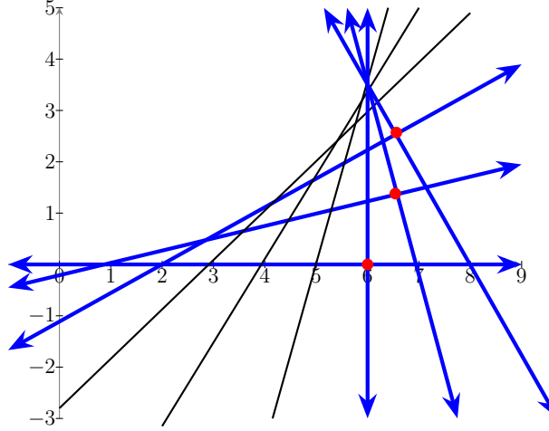
Figure 23: Dividing the plane into the maximum number of pieces using n \overline{X} 's (or coordinate frames). For n = 3 , draw a grid of lines \lambda_t defined by (9) with \theta = \pi/(4n) = \pi/12 and t = 0, \dots, 3n - 1 = 8 . The three \overline{X} 's (centered at the red dots, and with blue axes) are \lambda_0 \cup \lambda_6 , \lambda_1 \cup \lambda_7 , and \lambda_2 \cup \lambda_8 . An enlargement of the figure will show that, although it is not clear from this illustration, there is no point where any three of the lines intersect.
