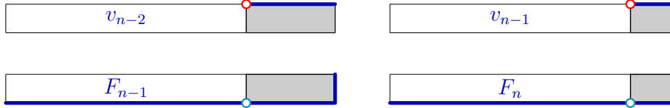
Figure 2: Tiling and walks on a (1 \times n) -board (reproduced from Németh [14]).
