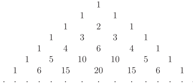
Figure 1: Pascal's triangle.
