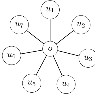
Figure 6: The star graph \mathcal{S}(7) with 7 edges
