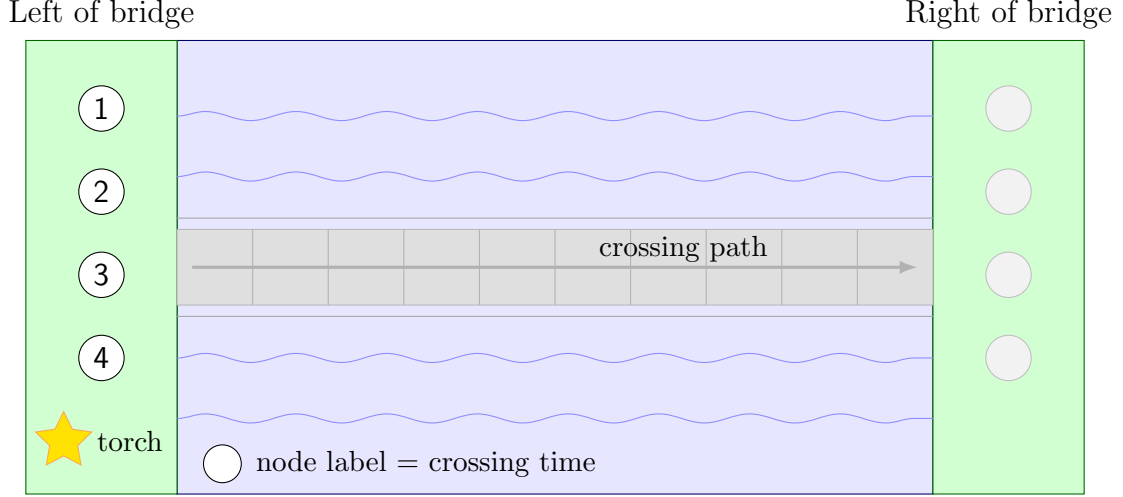
Figure 1: Visualizing the bridge and torch problem
