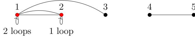
Figure 3: Visualizing the set of moves to obtain T(5)
