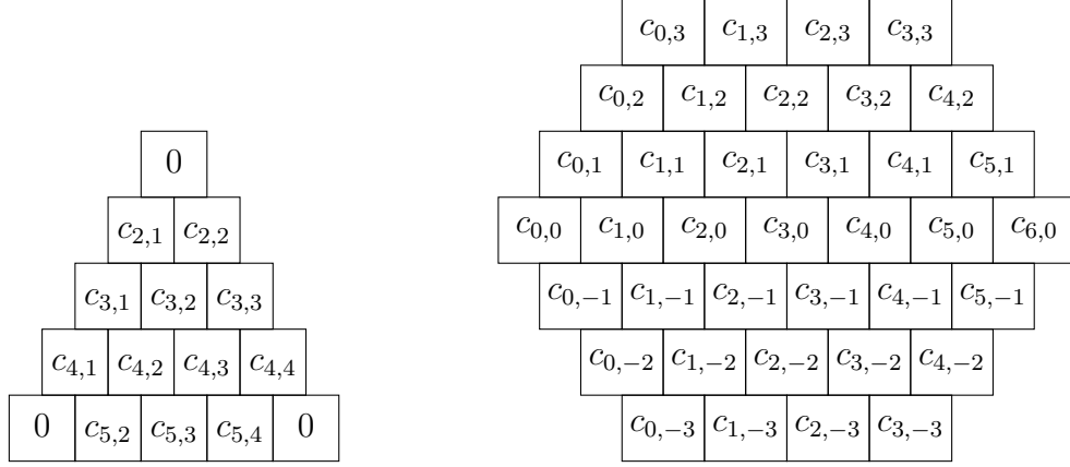
Figure 3: Illustrations of the arrays appearing in the definitions of A195806 (left) and A216940 (right), respectively.
