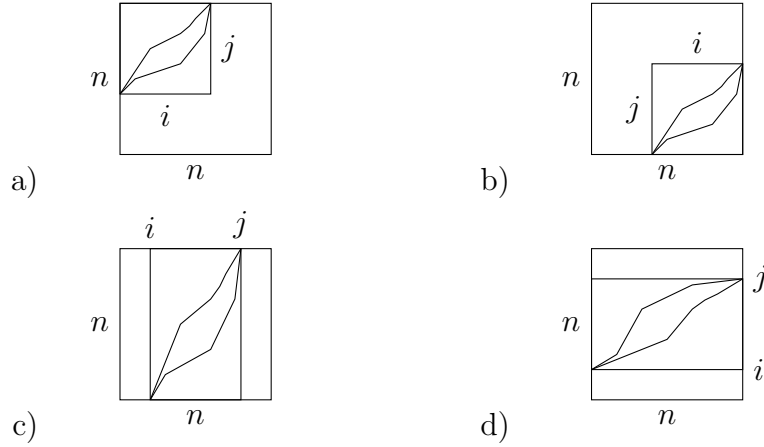
Figure 2: Case distinction used in the analysis of A306322 .
