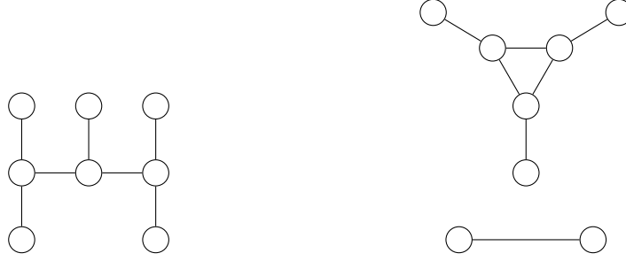
Figure 4: Two graphs with 8 vertices used for illustrating the definition of A339987 .
