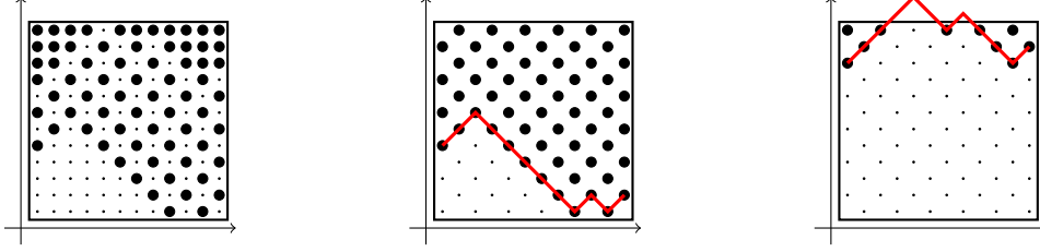
Figure 1: A particular 12 \times 12 array for A188818 (left), where dots and bullets represent 0's and 1's, respectively. The middle (resp., right) image shows the even (resp., odd) positions, where 0's and 1's are separated by a generalized Dyck path.
