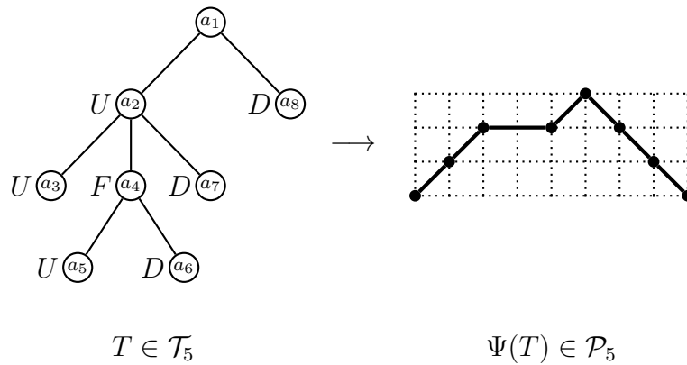
Figure 3: Illustrating the tree-to-path mapping \Psi (Definition 1)
