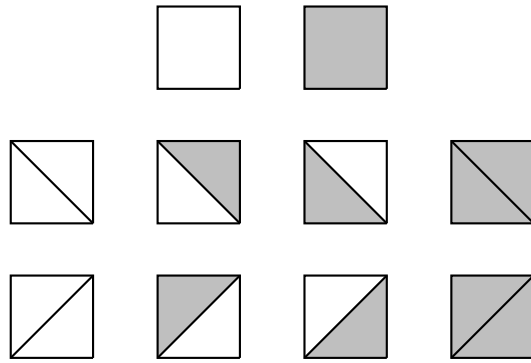
Figure 6: The s_2(3) = 10 ways to 2-color subdivisions of a square
