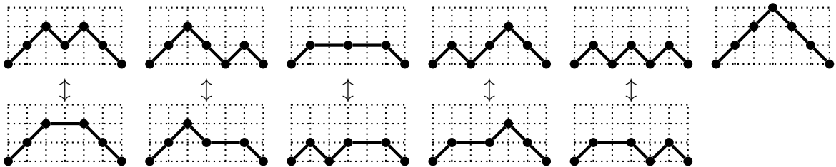
Figure 4: Illustrating our combinatorial proof of Proposition 6. Paths on the first (resp., second) row have an odd (resp., even) number of up steps.
