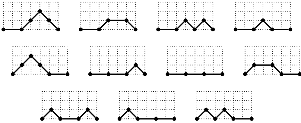
Figure 5: The 11 large Schröder paths in \overline{\mathcal{P}}_4 \setminus \mathcal{P}_4
