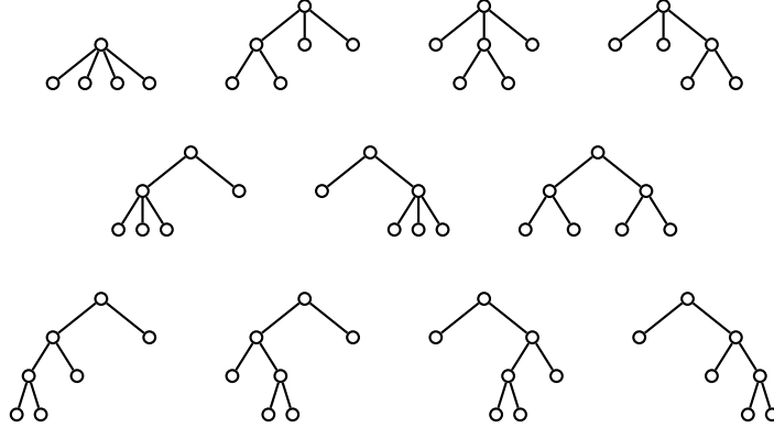
Figure 1: The s(4) = 11 Schröder trees with 4 leaves
