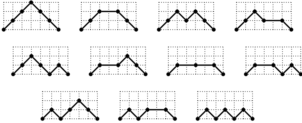
Figure 2: The s(4) = 11 small Schröder paths from (0,0) to (6,0)
