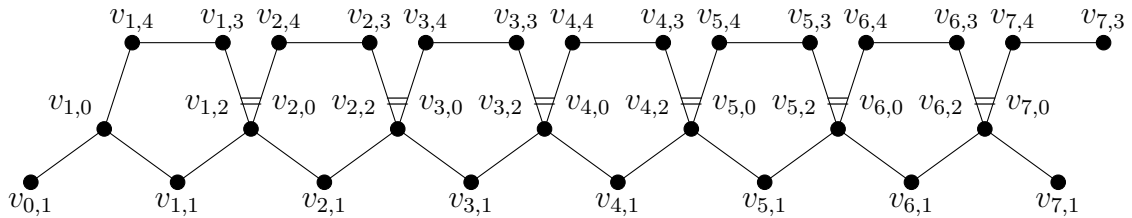
Figure 21: The fourth variation of the (2,6) -linked 5-cycle ^-(C_5)_{2,6}^\square
