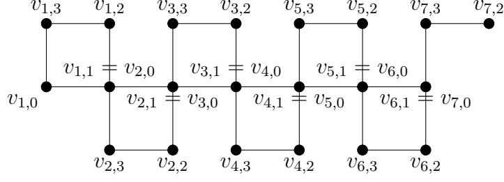
Figure 23: The first variation of the (1, 6) -linked 4-cycle (C_4)_{1,6}^{\vee}
