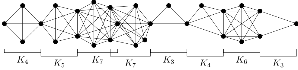
Figure 11: An 8-linked clique that links up K_4, K_5, K_7, K_7, K_3, K_4, K_6, K_3
