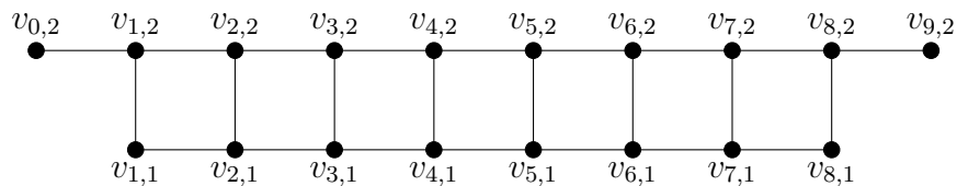
Figure 8: The second variation of the lattice graph {}^-L_{8 \times 2}^-
