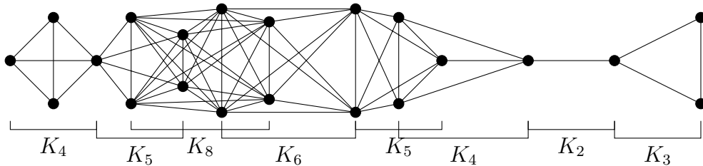
Figure 10: An 8-chained clique that chains up K_4, K_5, K_8, K_6, K_5, K_4, K_2, K_3
