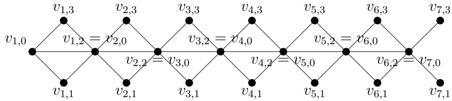
Figure 27: The first variation of the 6-linked diamond D_6^<
