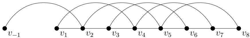
Figure 4: The B -version of a 3-path P_8^B(3)
