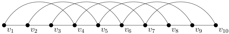
Figure 3: The 3-graph P_{10}(3)
