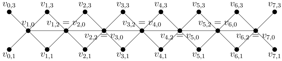
Figure 28: The second variation of the 6-linked diamond >D_6^<
