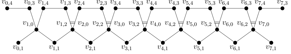
Figure 22: The fifth variation of the (2,6) -linked 5-cycle \sqsupset(C_5)_{2,6}^{\square}
