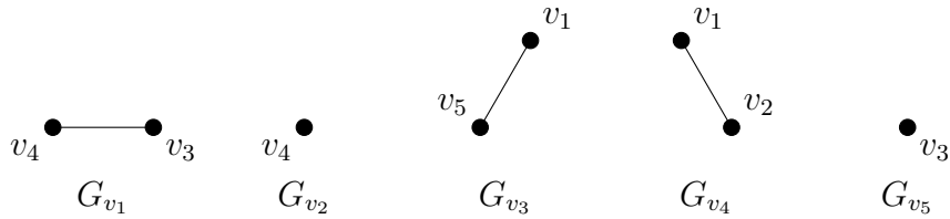
Figure 2: The residue subgraphs G_{v_1} , G_{v_2} , G_{v_3} , G_{v_4} , and G_{v_5}
