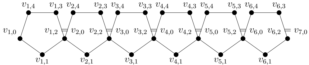
Figure 17: The (2, 6) -linked 5-cycle (C_5)_{2,6}
