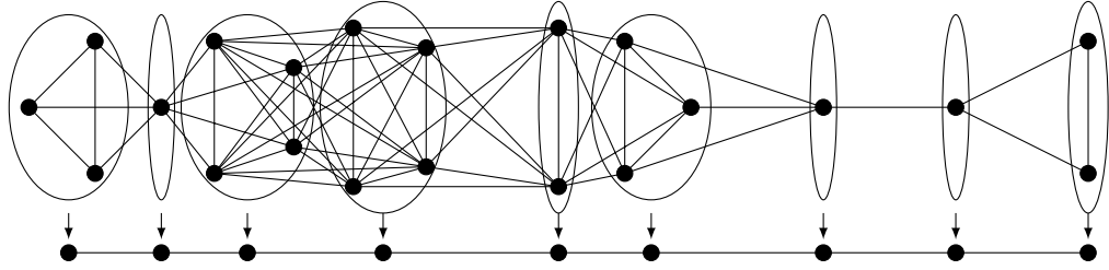
Figure 12: Transforming a CK_8 to P_9
