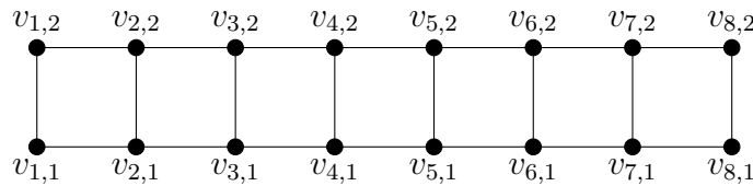
Figure 6: The lattice graph L_{8 \times 2}
