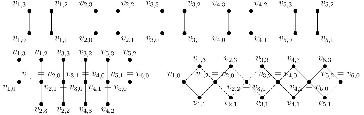
Figure 14: Linking 5 copies of C_4 (top) as (C_4)_{1,5} (bottom left) or (C_4)_{2,5} (bottom right)
