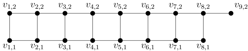
Figure 7: The first variation of the lattice graph L_{8 \times 2}^-
