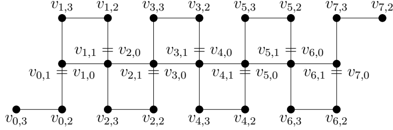
Figure 24: The second variation of the (1, 6) -linked 4-cycle {}^{\vee}(C_4)_{1,6}^{\vee}
