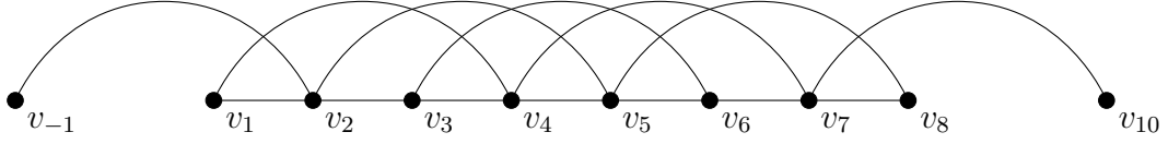
Figure 5: The C -version of a 3-path P_8^C(3)
