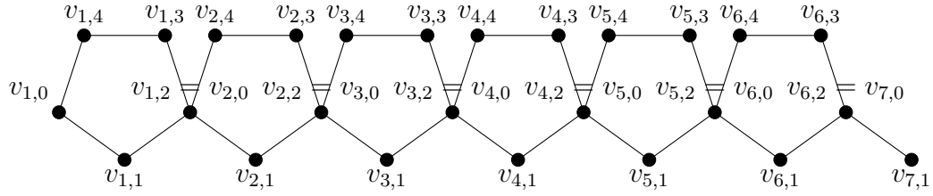
Figure 18: The first variation of the (2,6) -linked 5-cycle (C_5)_{2,6}^-
