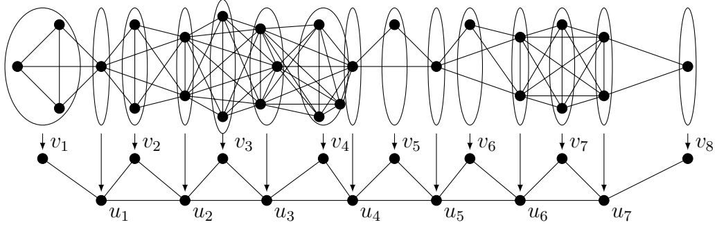
Figure 13: Transforming an LK_8 to T_8
