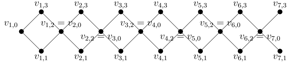
Figure 15: The first variation of the (2, 6) -linked 4-cycle (C_4)_{2,6}^<
