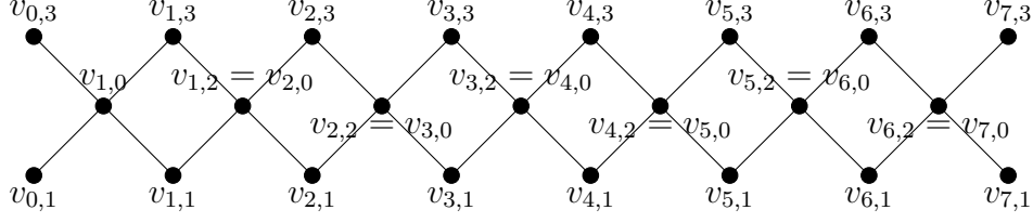
Figure 16: The second variation of the (2, 6) -linked 4-cycle \succ(C_4)_{2,6}^{\leq}
