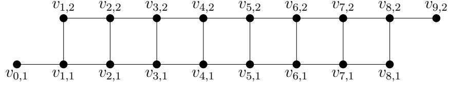
Figure 9: The third variation of the lattice graph -L_{8 \times 2}^{-}
