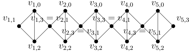
Figure 26: A 2n -chained clique CK_{2n}
