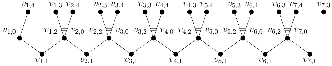
Figure 19: The second variation of the (2,6) -linked 5-cycle (C_5)_{2,6}^\square
