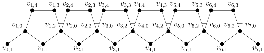
Figure 20: The third variation of the (2,6) -linked 5-cycle ^-(C_5)_{2,6}^-
