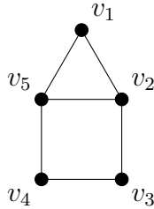
Figure 1: A simple graph G
