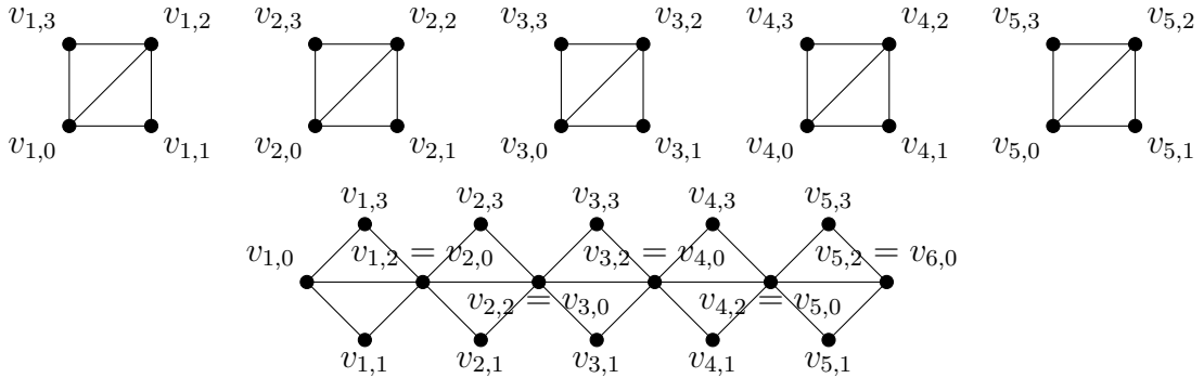
Figure 25: Linking 5 diamonds (top) as D_5 (bottom)
