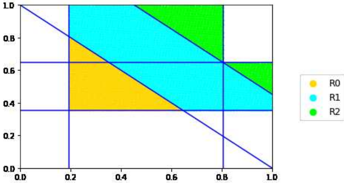
Figure 1: The regions R_0 , R_1 , and R_2 in the uv -plane representing the conditions given in Proposition 21 for the perturbation errors c(n) - \tilde{c}(n) to be equal to 0, 1, and 2, respectively. The vertical boundary lines are given by the equations u = \alpha and u = 1 - \alpha , the horizontal boundary lines are given by the equations v = \beta , v = 1 - \beta , and the two diagonal lines are given by u + v = 1 and u + v = 1 + \gamma .
