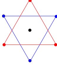
Figure 3: Vertical star of David.
