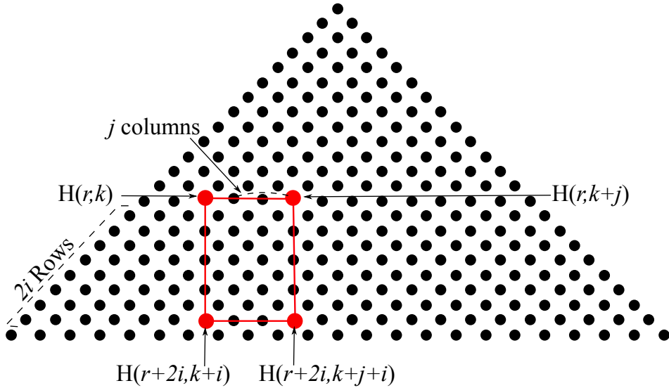
Figure 4: Property of Rectangle.
