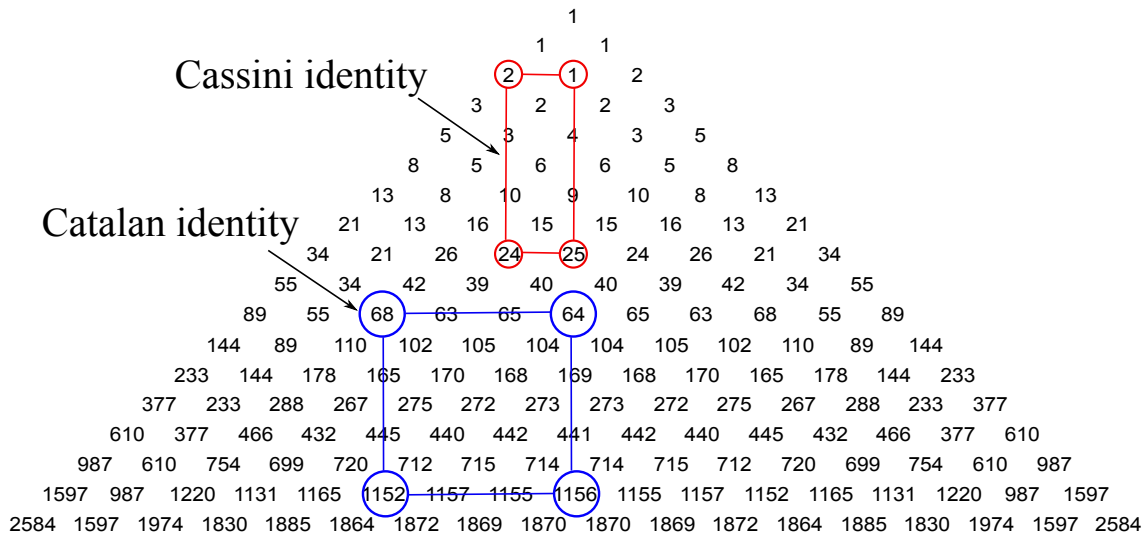
Figure 5: Cassini and Catalan identities in the Hosoya Triangle.
