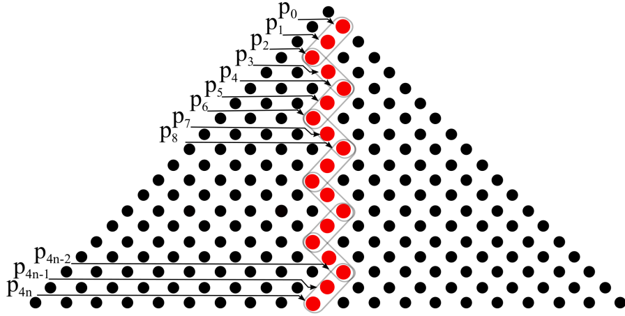
Figure 7: Geometric interpretation of Corollary 16.
