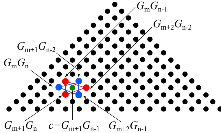
Figure 2: Star of David in a Hosoya triangle where G_k is either \mathcal{F}_k or \mathcal{L}_k for all k \geq 0 .
