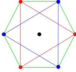
Figure 1: Star of David from a hexagon.
