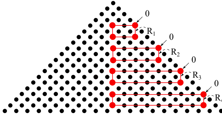
Figure 6: Geometric interpretation of Theorem 15.
