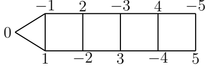
Figure 1: Graph G_{11}
