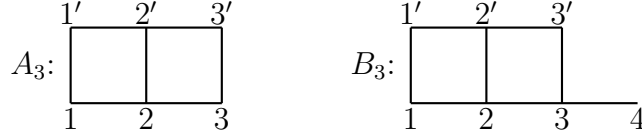
Figure 2: Graphs A_3 and B_3
