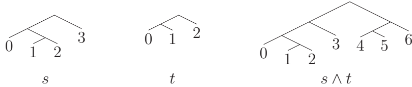
Figure 1: A binary operation on binary trees
