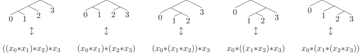
Figure 2: Correspondence between binary trees and parenthesizations
