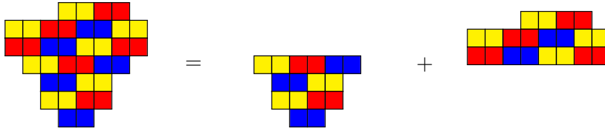
Figure 2: Dividing a convex (18, 4) -domino tower
