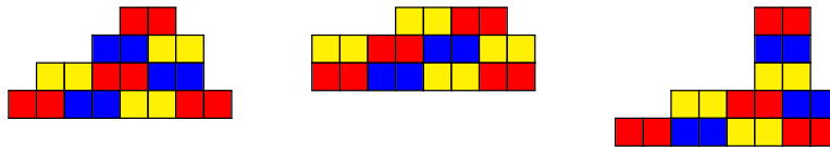
Figure 4: Examples of (10, 4) -domino stacks
