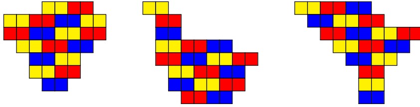
Figure 1: Examples of convex (18, 4) -domino towers
