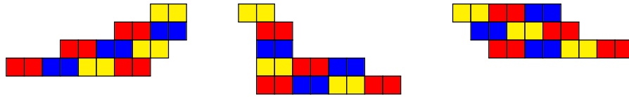
Figure 5: Examples of right-skewed or left-skewed (10, 4) -domino towers
