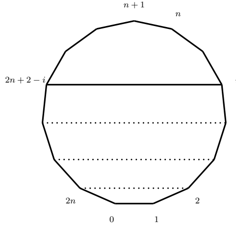
Figure 3: Illustration of the proof of (7).
