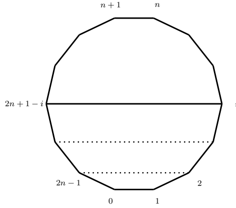
Figure 2: Illustration of the proof of (5). The dotted lines represent the avoided diagonals.
