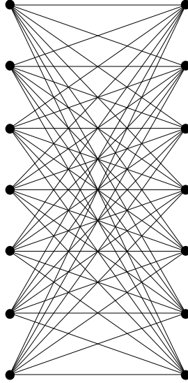
Figure 1: A regular drawing of the complete bipartite graph K_{7,7} .
