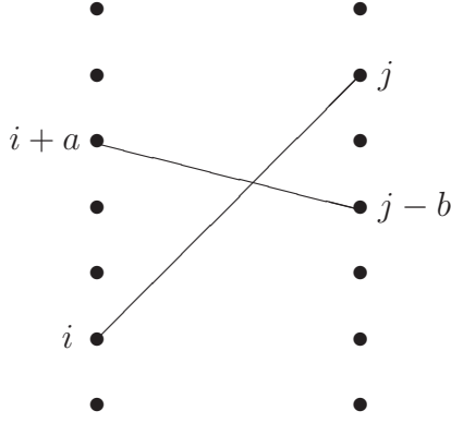
Figure 2: An (a, b) crossing with a = 3 , b = 2 , i = 2 , j = 6 and k = 1 .
