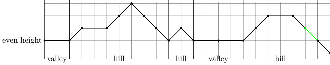
Figure 6: Partitioning the first active subpath into hills and valleys. The second active subpath is the rightmost hill or valley with a horizontal step.
