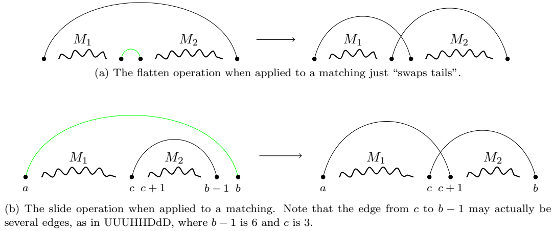
Figure 8: The effect of e on matchings. This is the matchings version of Figure 3.
