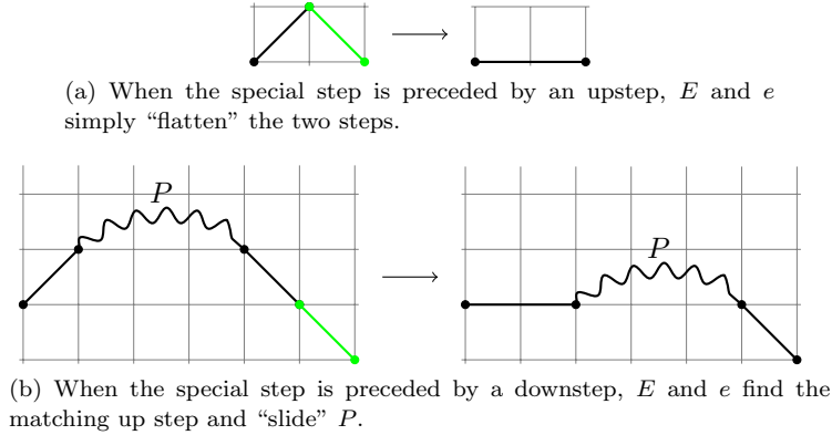
Figure 3: The action of bijections E and e on the leftmost special down step in a hybrid path.
