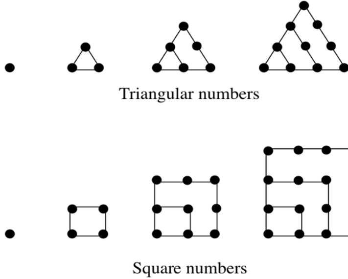
Figure 1: Geometrical Representation of Polygonal Numbers
