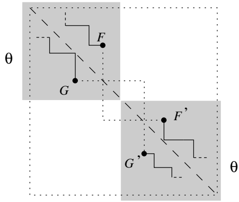
FIGURE 12. If \pi = \theta \ominus \theta' then the boundary of every polygon associated with \pi crosses itself.
