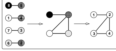
FIGURE 1. The graph associated to the coloured set partition \{\{1_3, 4_2\}, \{2_2, 6_4\}, \{3_4, 7_3\}, \{5_2, 8_1\}\}
