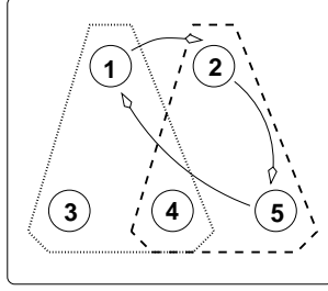
FIGURE 2. A structure composed of a set of smaller structures (cycles and 3-sets).
