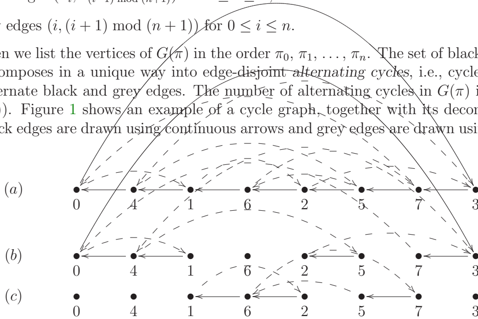
Figure 1: (a) The cycle graph of \langle 4\ 1\ 6\ 2\ 5\ 7\ 3 \rangle ; (b), (c) its decomposition into two alternating cycles
