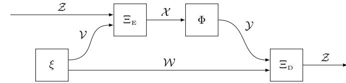
Figure 8.1 An illustration of the map Z \mapsto (\Xi_D(\Phi \Xi_E \otimes \mathbf{1}_{L(\mathcal{W})}))(Z \otimes \xi) referred to in Definition 8.5.
