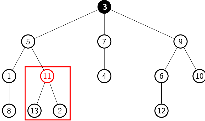
Figure 2.4: Tree-structured groups are simply rooted subtrees in a rooted tree. The red rectangle denotes the group induced by the subtree rooted at the red node.
