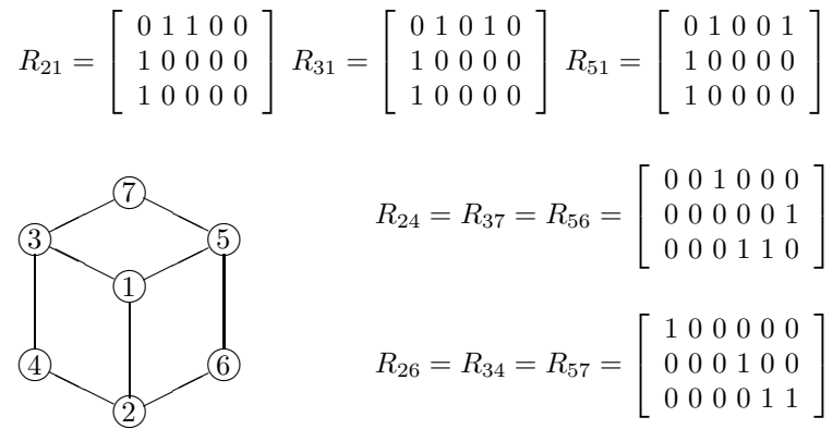
Figure 2: Scene labeling constraint network
