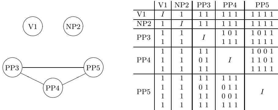
Figure 5: Left: Parsing constraint network; Right: Table representation of constraint network
