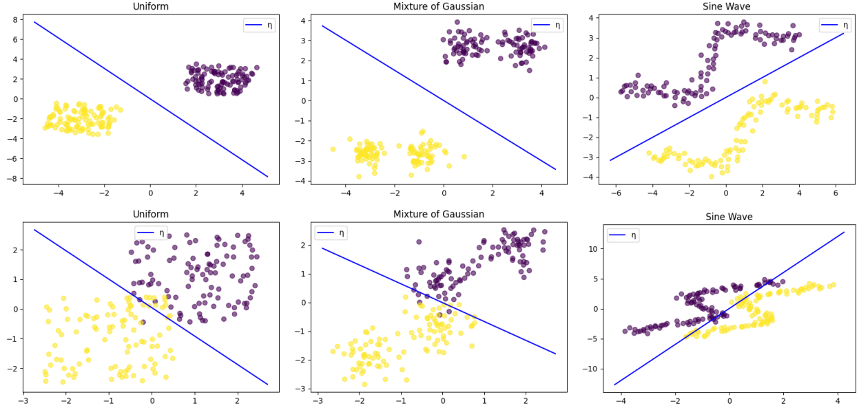
Figure A.3: Yellow and purple dots are data of two different classes. The blue line is the learned linear separator \eta .
