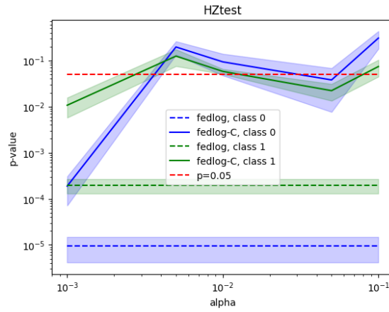
Figure A.2: HZtest results of the ablation study. Higher is better. Colored area show mean \pm standard error.
