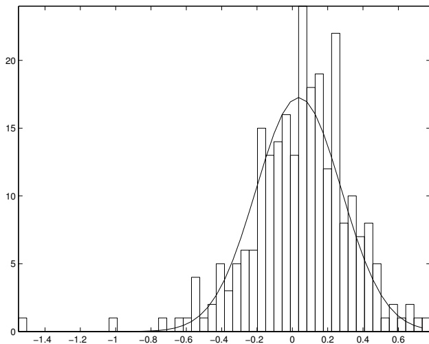
Figure: Scaled to zero mean and unit standard deviation, standard normal distribution also shown
