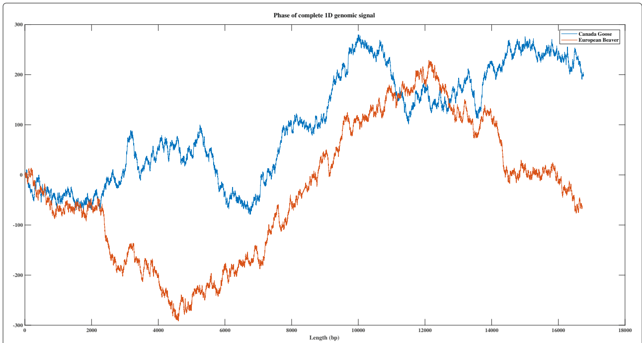
Fig. 2 Canada goose (blue, 16,760 bp) vs. European beaver (red, 16,722 bp) - comparison between the DFT phase spectra of their full mtDNA genomes
