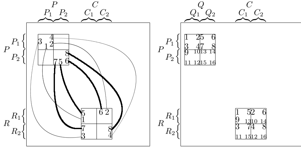
Fig. 5.1. All 8 possible smaller cases of invoking \text{REMOVE}(P_x, R_y, C_z) are shown on the left figure for the special problem. Each of them considers a pair of squares, which are indicated by the same number. The figure on the right shows 16 possible subroutines for \text{REMOVE}(P_w, Q_x, R_y, C_z) in general graphic matroid parity. Note that in the special problem the rows and the columns of the first square are the same, while in the general problem the rows and the columns of the first square could be different.
