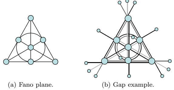
Figure 3: (a) The Fano plane is an intersecting hypergraph with 7 hyperedges of size 3. (b) The integrality gap example with k = 4 and q = 2 .
