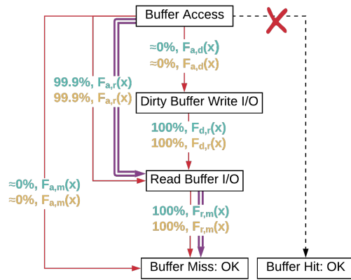
Figure 7: Combining empirical CDFs using random walks for Scenario A (blue) and Scenario B (orange) on a subset of the buffer access transition model. Crossed-out paths indicate those pruned from consideration. Double purple lines indicate the random walk example in the text. F_{e_1, e_2}(x) are CDFs for percentile x of transition times from event e_1 to event e_2 .
