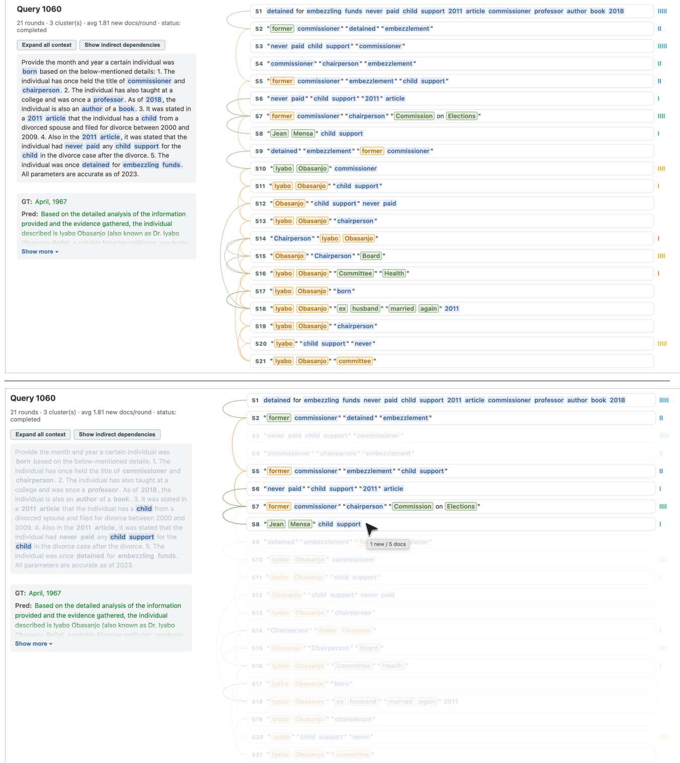
Figure 6: Demo of the detailed question page in HAWKEYE. Top: Default page display; Bottom: Highlighting the sources of the query tokens when a query entry is hovered over.
