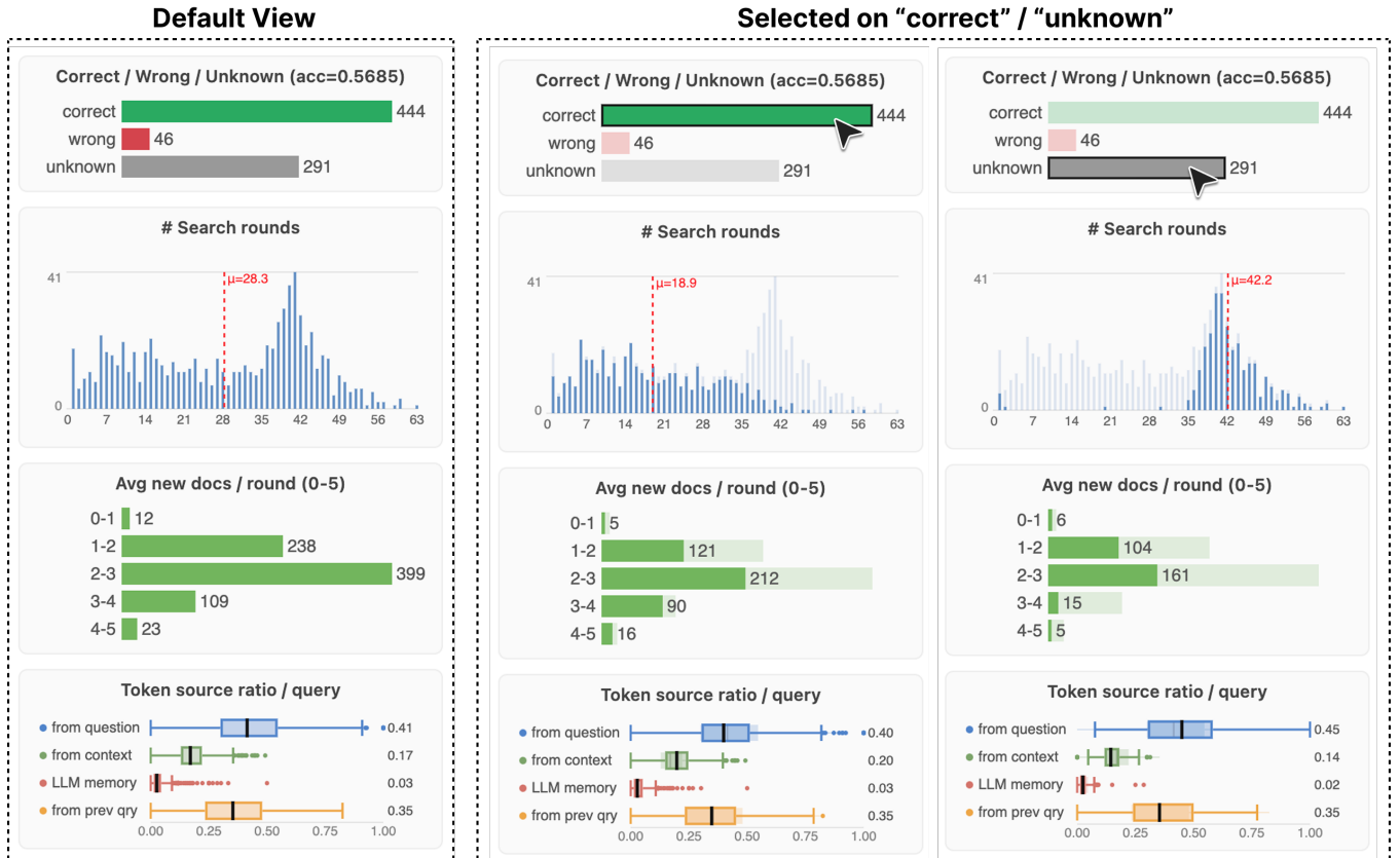
Figure 5: Demo of the detailed meta statistics panels in HAWKEYE. Left: Default meta statistics panels; Middle and Right: After selecting the “correct” or “unknown” categories in the first panel, the meta statistics panels are updated to the statistics of questions under the selected category. (Note: The differences after selection in Panel 4 may be easier to see when zoomed in due to the panel’s rich use of color.)
