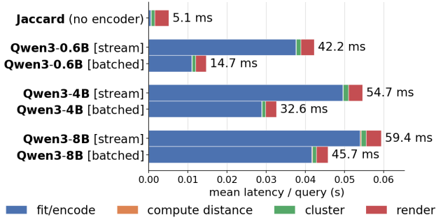
Figure 2: Breakdown of rendering latency per query. (Note that here the Qwen embedding models are used to compute pairwise query distance, and are independent from the retrievers used in the agentic search process.)
