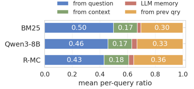
Figure 3: Aggregated query provenance ratios on BrowseComp-Plus while using Tongyi and three retrievers. Colors match to their corresponding category in the query provenance panel. “Qwen3-8B”: Qwen3-Embedding-8B, “R-MC”: Reason-ModernColBERT.
