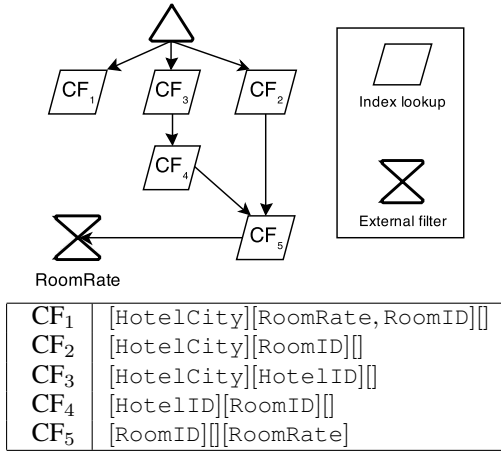
Fig. 6. Example query plan space
