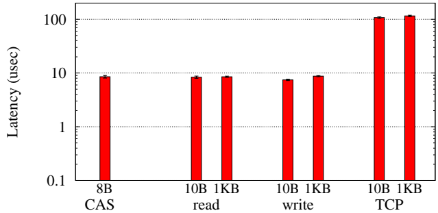
Figure 1: RDMA Latency
