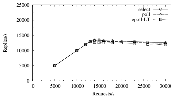
Figure 2: \mu server performance on SPECweb99-like workload using select , poll , and epoll-LT
